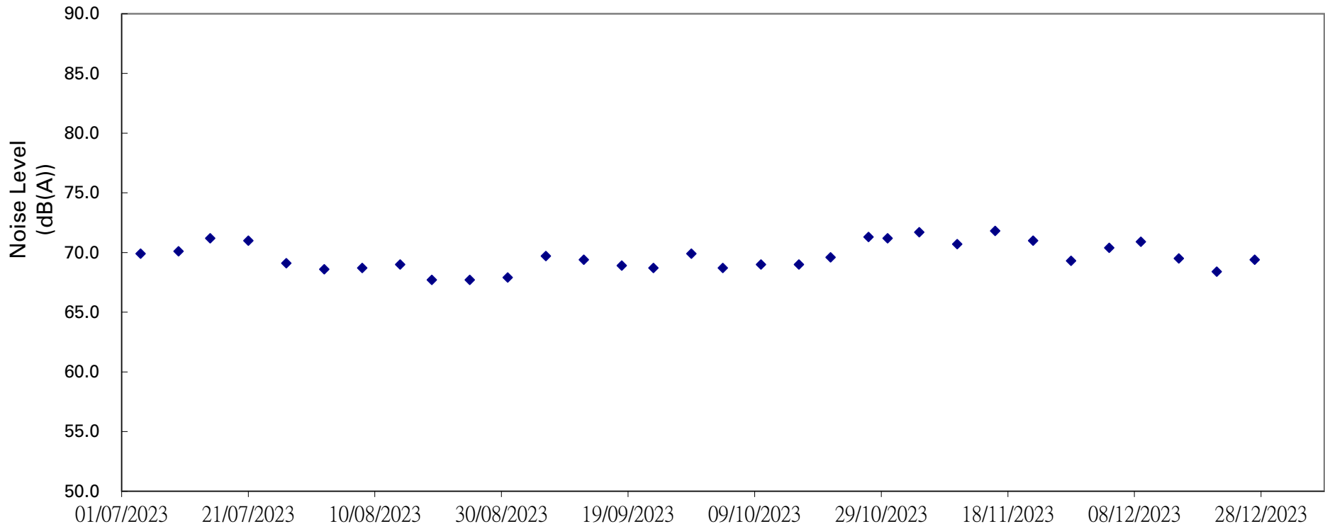
Noise Level (Leq 30 mins) dB(A) Vs Date for Location W-N18
